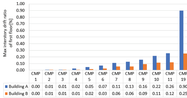
Figure 13. Graphical and numerical representation of the maximum interstory drift recorded at the first floor of both buildings during each test.
