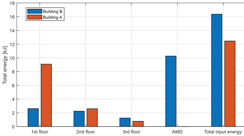
Figure 21. Energy balance in both buildings (test CMP 19).
