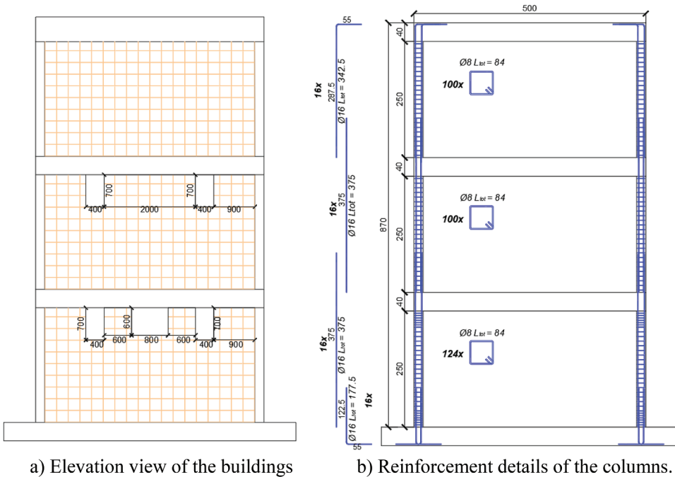
Figure 3. a) Elevation view of the buildings; b) Reinforcement details of the columns.
