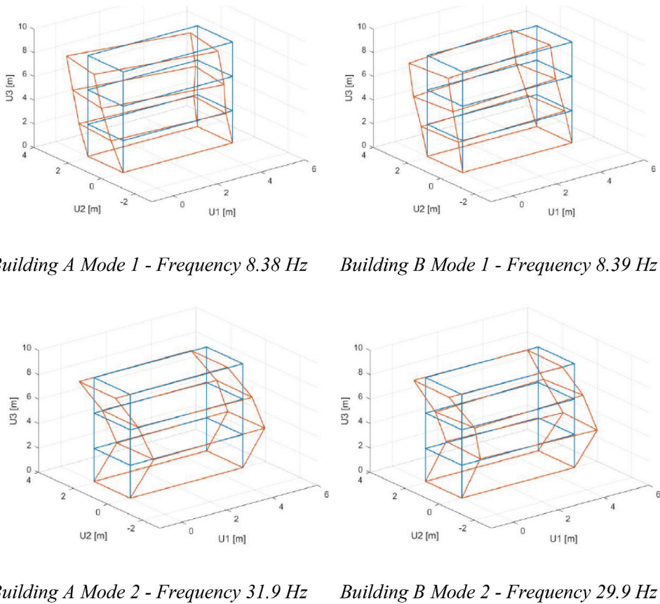
Figure 10. First and second modes from experimental modal analysis. Building A Mode 1 – Frequency 8.38 Hz Building B Mode 1 – Frequency 8.39 Hz Building A Mode 2 – Frequency 31.9 Hz Building B Mode 2 – Frequency 29.9 Hz.
