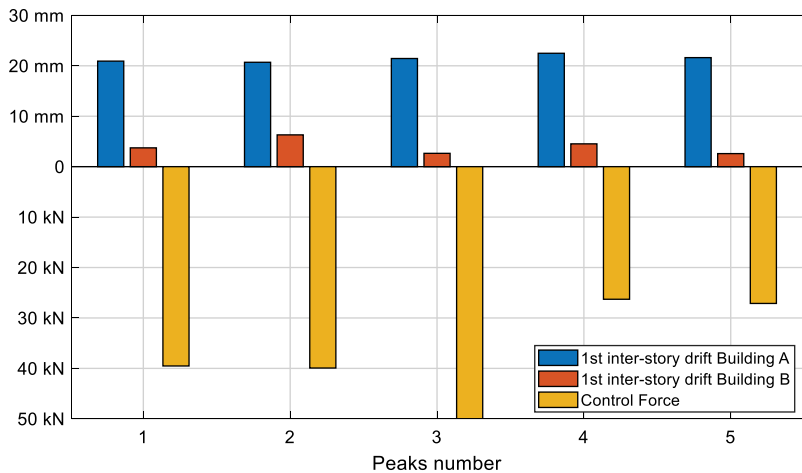
Figure 15. Five largest first floor inter-story drifts (Buildings A and B) and corresponding AMD forces (Building B) recorded during test CMP 19.
