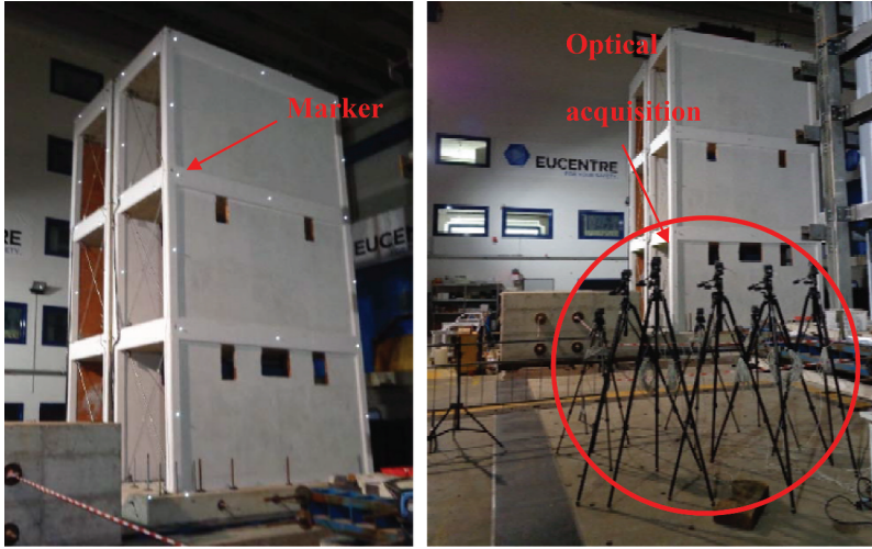
Figure 9. Markers and optical acquisition system.
