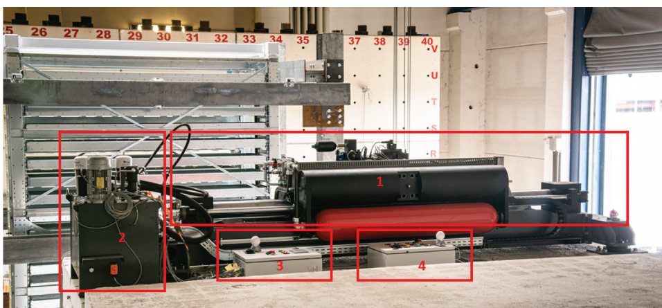
Figure 2. The AMD proposed: 1) hydraulic cylinder; 2) oil restoration control unit; 3) control panel and fault management; 4) control panel and fault management of hydraulic control unit.
