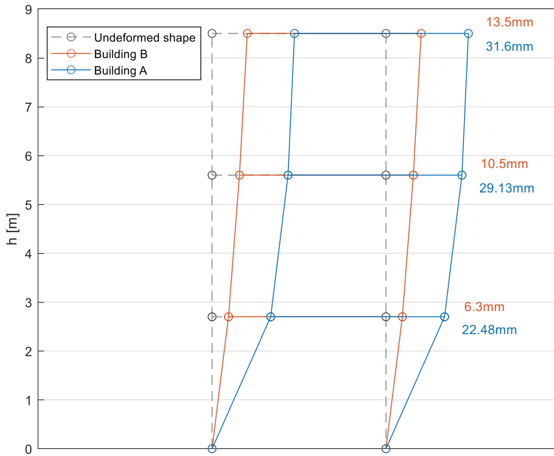
Figure 16. Maximum displacement envelope for both buildings (CMP 19).
