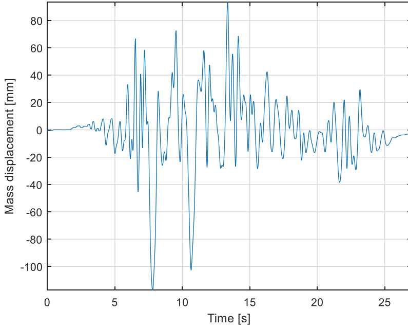
Figure 17. AMD Mobile mass displacement during test CMP 19.
