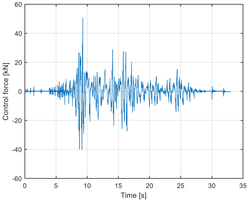
Figure 18. Control force generated by the AMD during test CMP 19.
