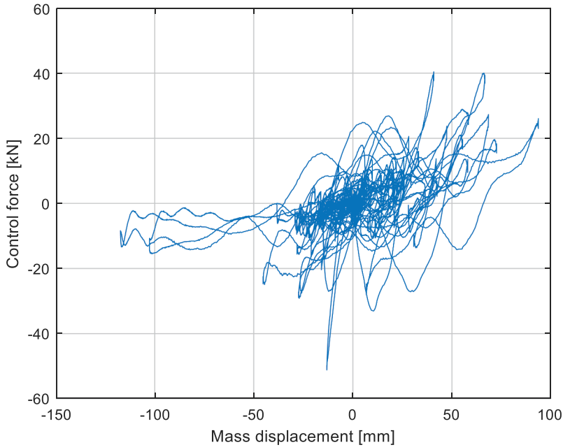
Figure 19. Relationship between control force and mobile mass displacements during test CMP 19.
