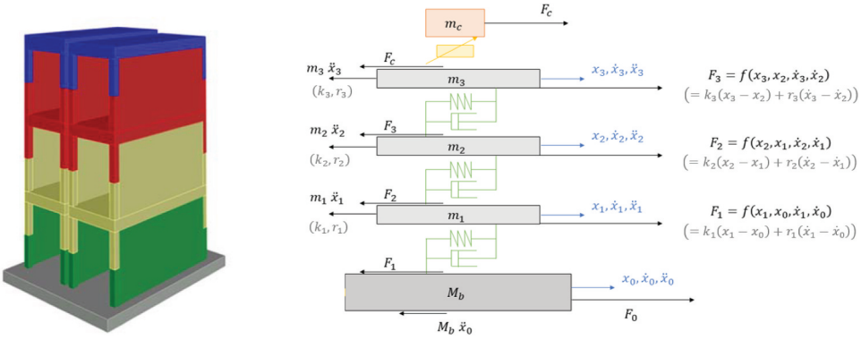
Figure 20. Lumped-element model of the building.
