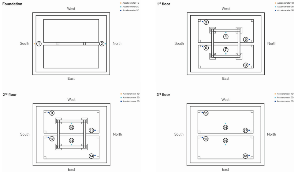
Figure 6. Accelerometers arrangement at the various levels.
