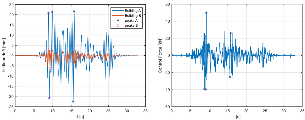
Figure 14. First floor inter-story drift for both buildings (left) and AMD control force (right) during test (CMP 19).
