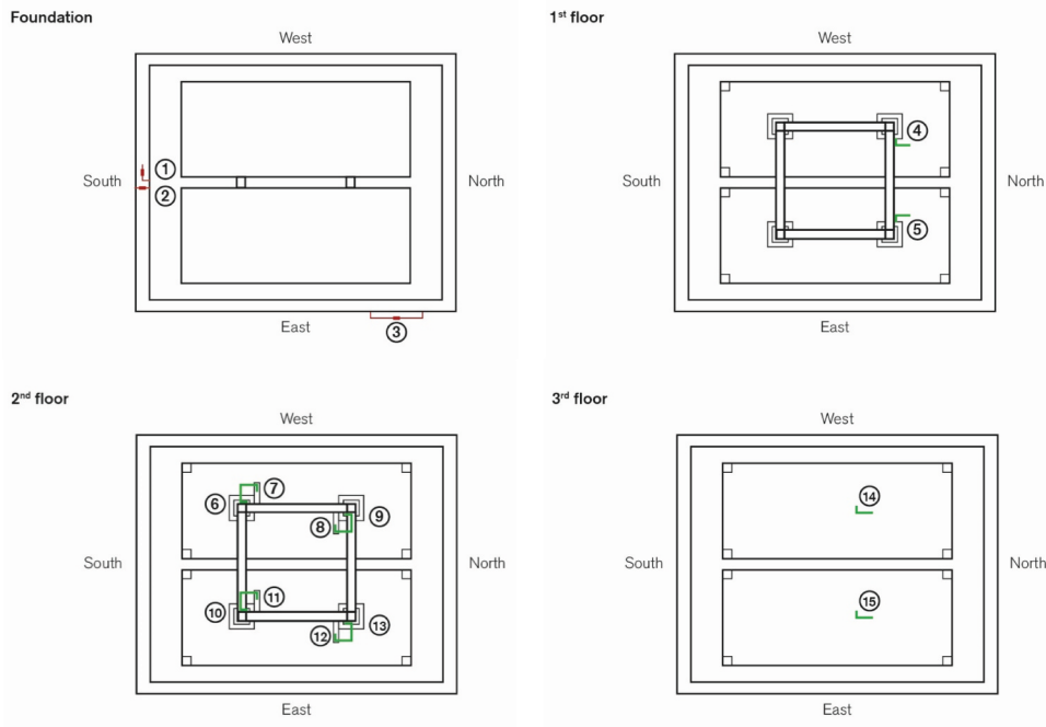
Figure 7. Displacement transducers arrangement at the various levels.
