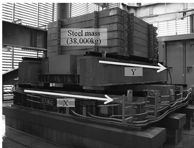
Figure 1. Application example of an active mass damper (Yamamoto and Sone 2014).
