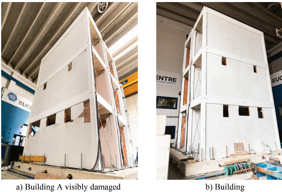
Figure 11. Damage in the buildings after test CMP19: a) Building A visibly damaged, b) Building B virtually undamaged.
